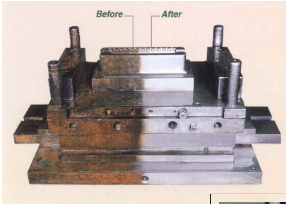
Mold cleaned with Rosler Wetblast unit
