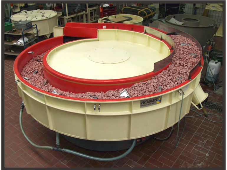
The R 400/9 LR, featuring 29 feet of processing in a single pass
