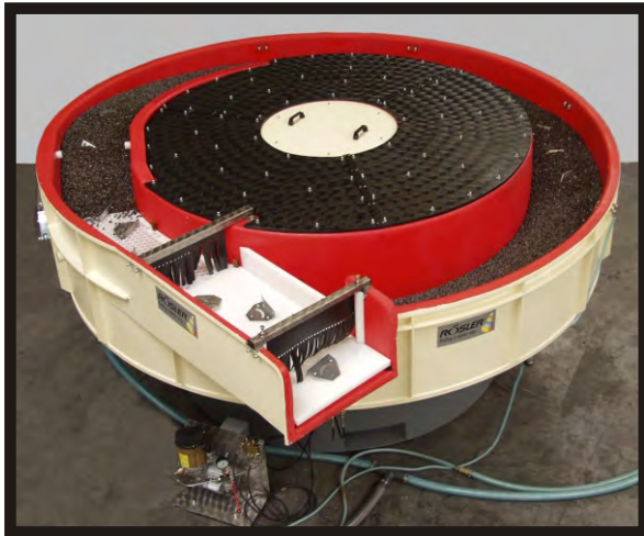
The R 310/5 LR, designed with continuous flow processing in mind
